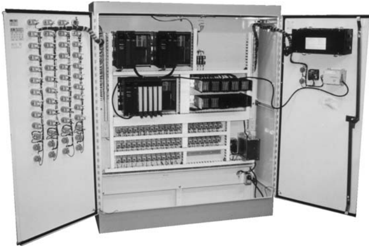
PLC driven Constant Level Control for two remote VFD's
